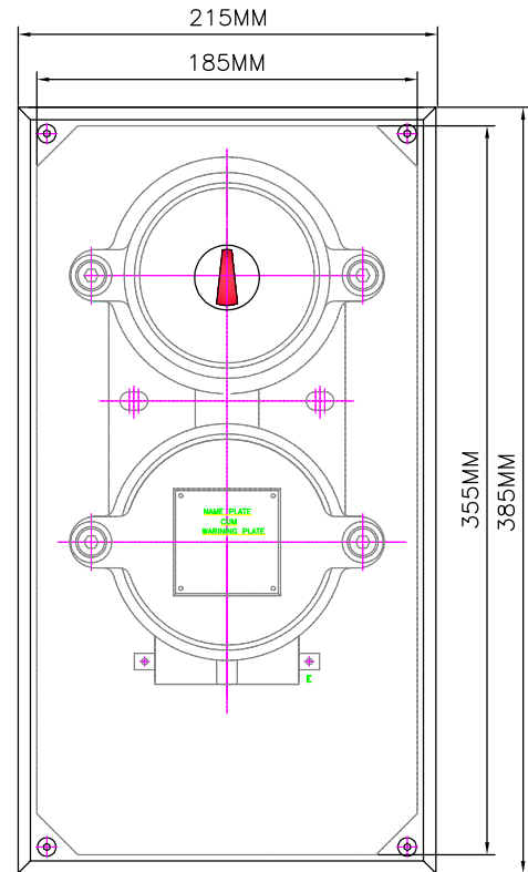
DEPTH 150MM
